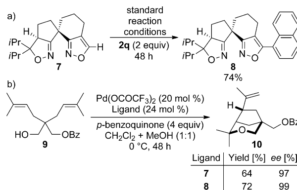
Scheme 4. Application of the direct arylation of isoxazoles.
