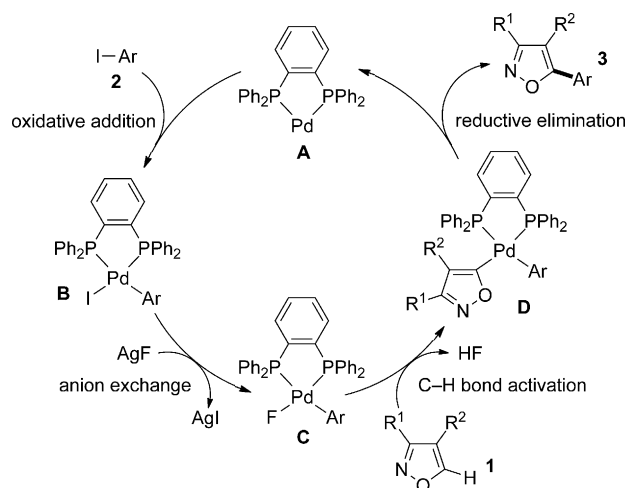
Scheme 2. Plausible catalytic cycle.
