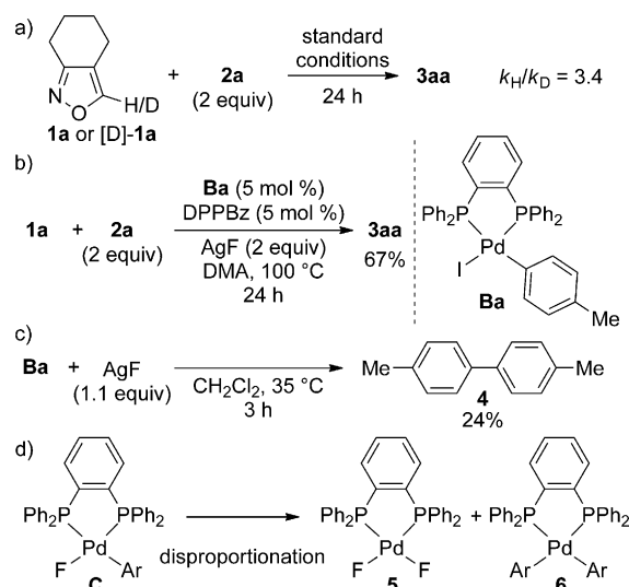
Scheme 3. Mechanistic study.
